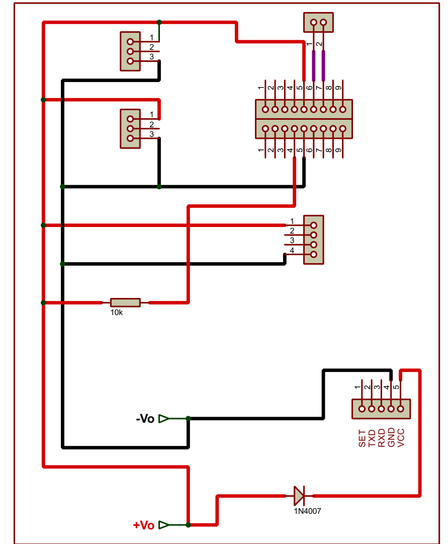
BACK BOARD
